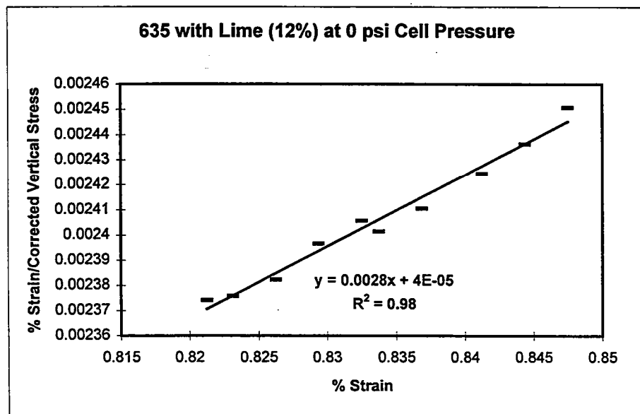
Figure 16. Modified Plot for Lime (12%) at 0 psi Cell Pressure (IH 635)
