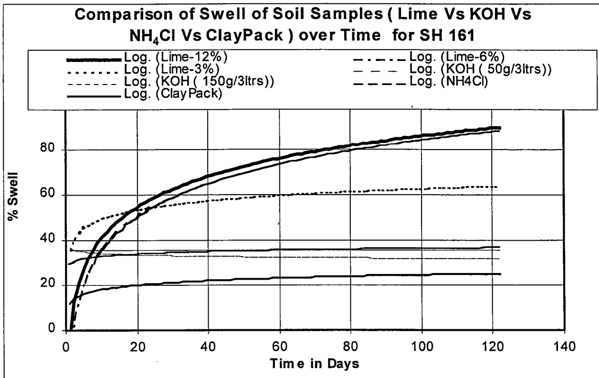
Figure 28. Comparison of Swell of Soil Samples (Lime Vs KOH Vs \text{NH}_4\text{Cl} Vs ClayPack) for SH 161
