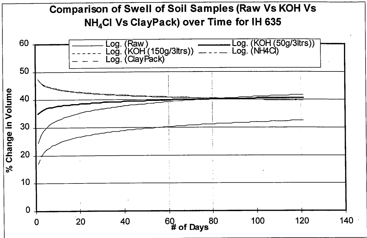
Figure 38. Comparison of Swell of Soil Samples (Raw Vs KOH Vs NH 4 Cl Vs ClayPack) for IH 635
