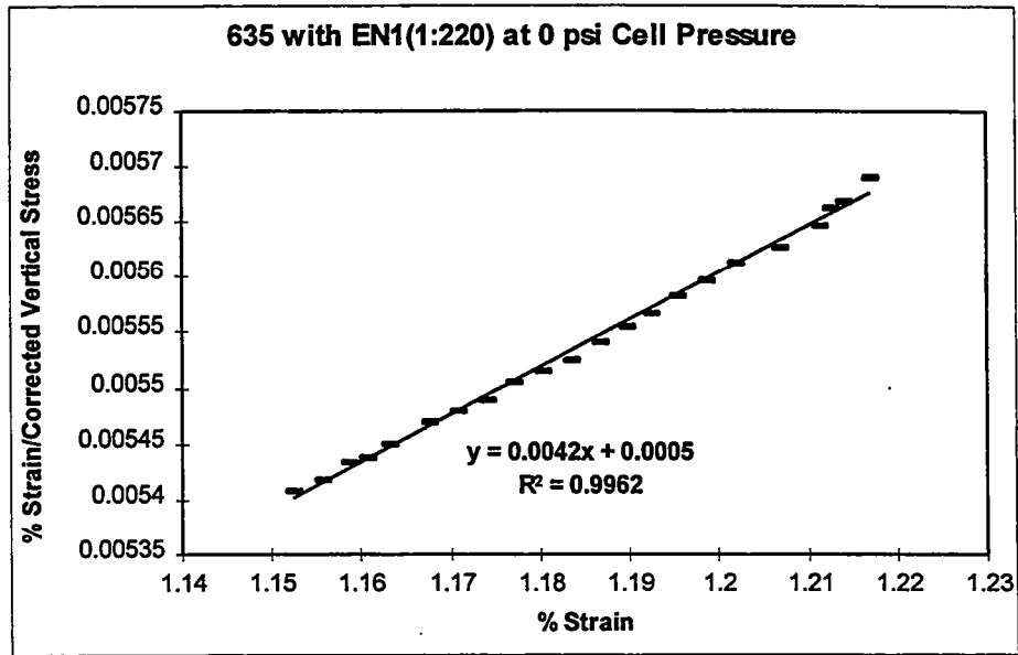
Figure 19. Modified Plot for EN1 (1:220) at 0 psi Cell Pressure (SH 161)
