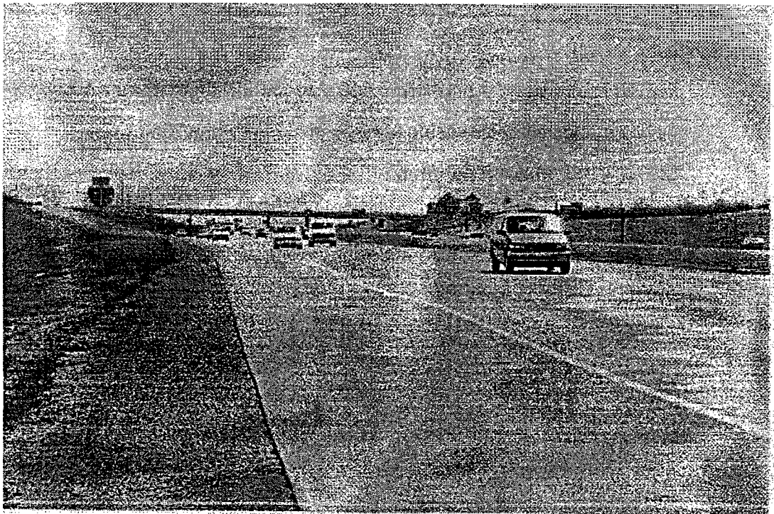
Figure 13. Sections of IH 635 Experiencing Heaving
