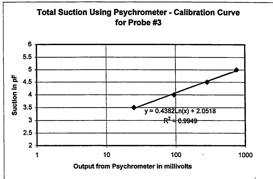
Figure 31. Calibration Chart for Probe #3
