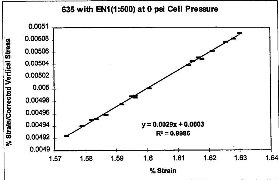
Figure 23. Modified Plot for EN1 (1:500) at 0 psi Cell Pressure (IH 635)
