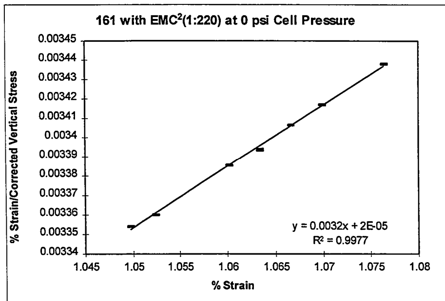
Figure 6. Modified Plot for EMC 2 (1:220) at 0 psi Cell Pressure (SH 161)
