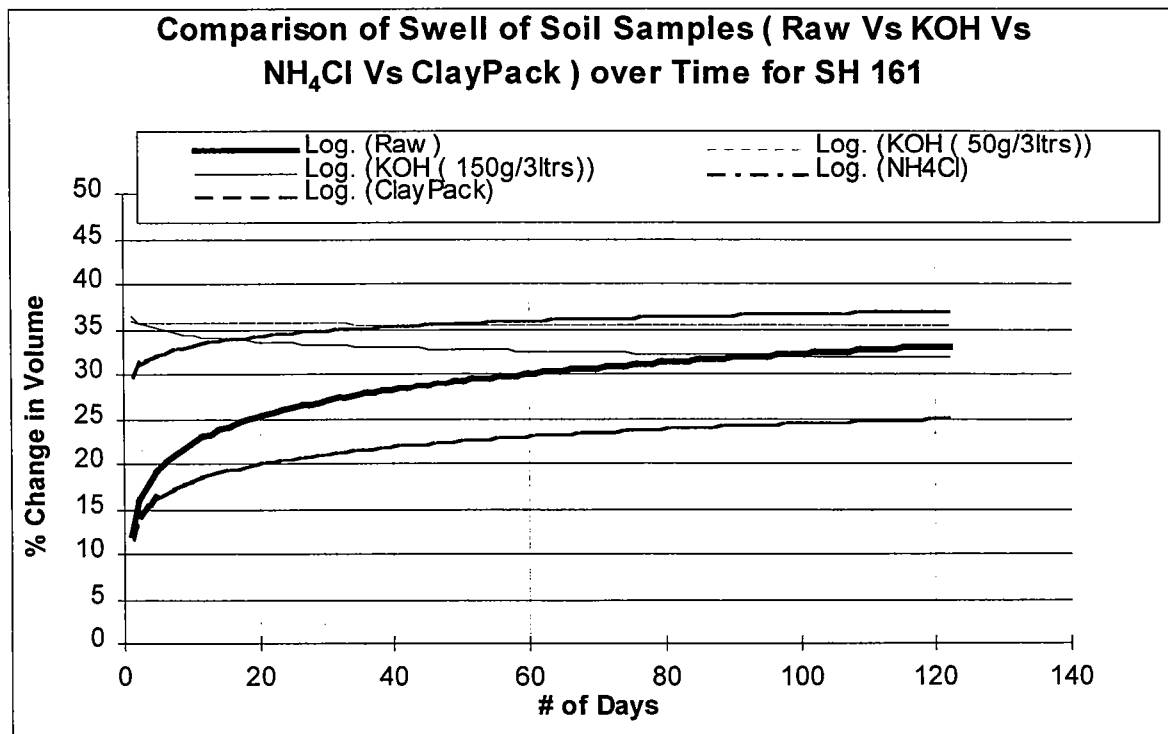
Figure 29. Comparison of Swell of Soil Samples (Raw Vs KOH Vs \text{NH}_4\text{Cl} Vs ClayPack) for SH 161
