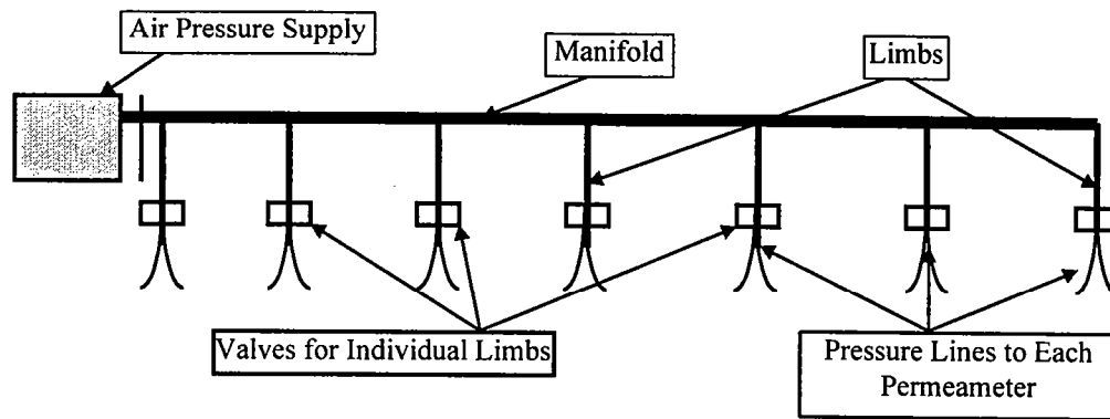
Figure 20. Schematic of Permeameter Setup
