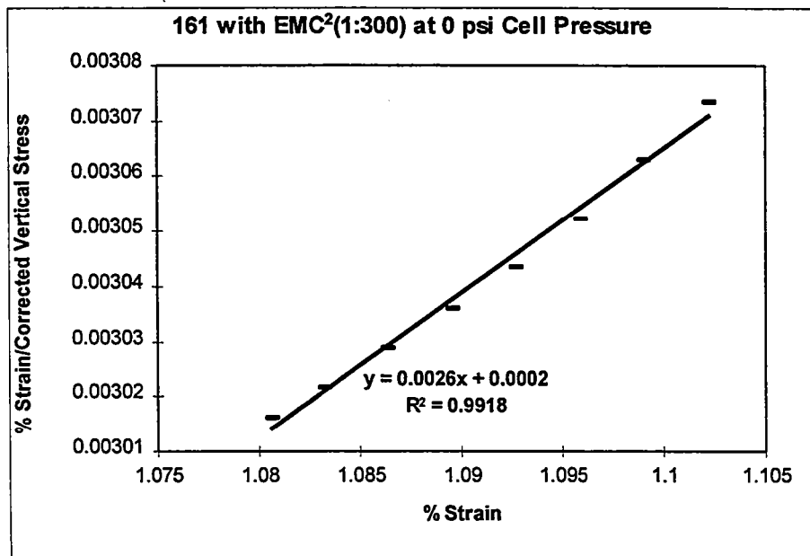
Figure 8. Modified Plot for EMC 2 (1:300) at 0 psi Cell Pressure (SH 161)
