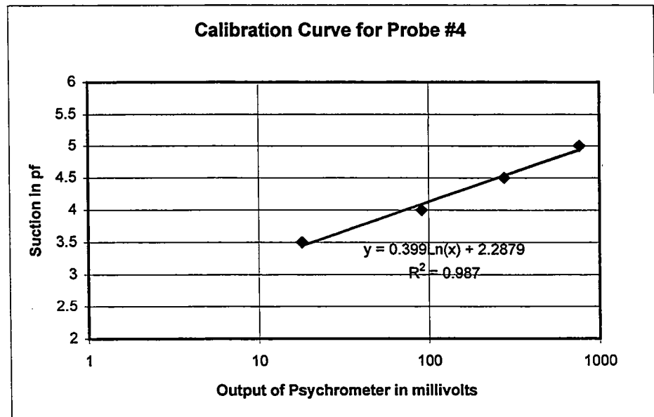
Figure 32. Calibration Chart for Probe #4
