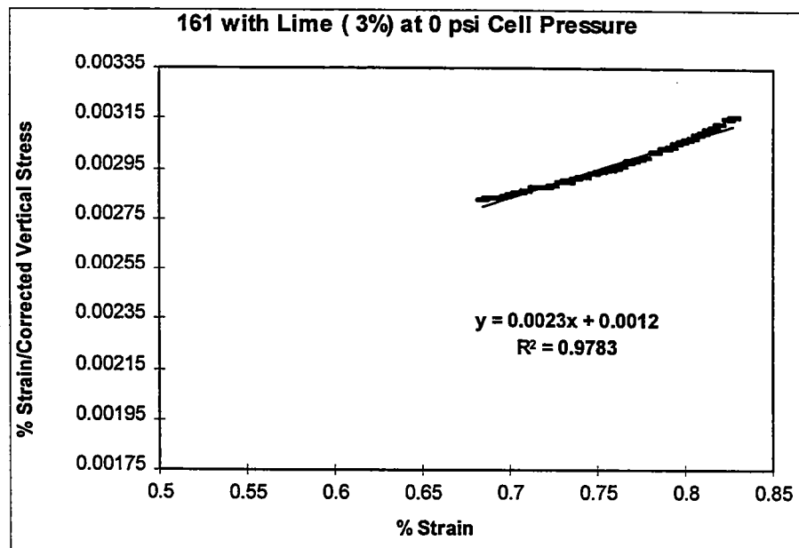
Figure 4. Modified Plot for Lime (3%) at 0 psi Cell Pressure (SH 161)
