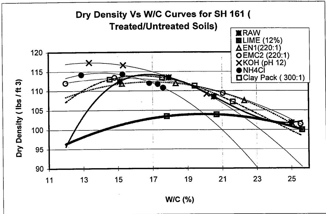
Figure 15. Dry Density Vs W/C Curves for SH 161
