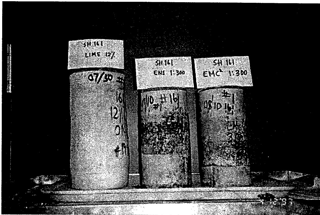
Figure 40. Photographs Showing Comparisons of Swell (Lime -12% Vs EN1-1:300, EMC²-1:300) - SH 161
