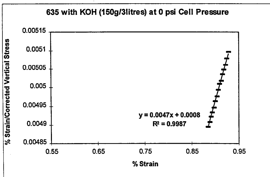
Figure 26. Modified Plot for KOH (150g/3ℓ) at 0 psi Cell Pressure (IH 635)
