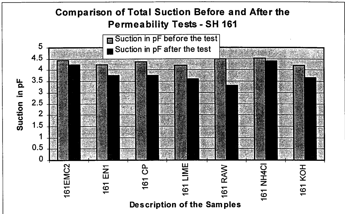
Figure 60. Comparison of Total Suction Before and After the Permeability Tests - SH 161
