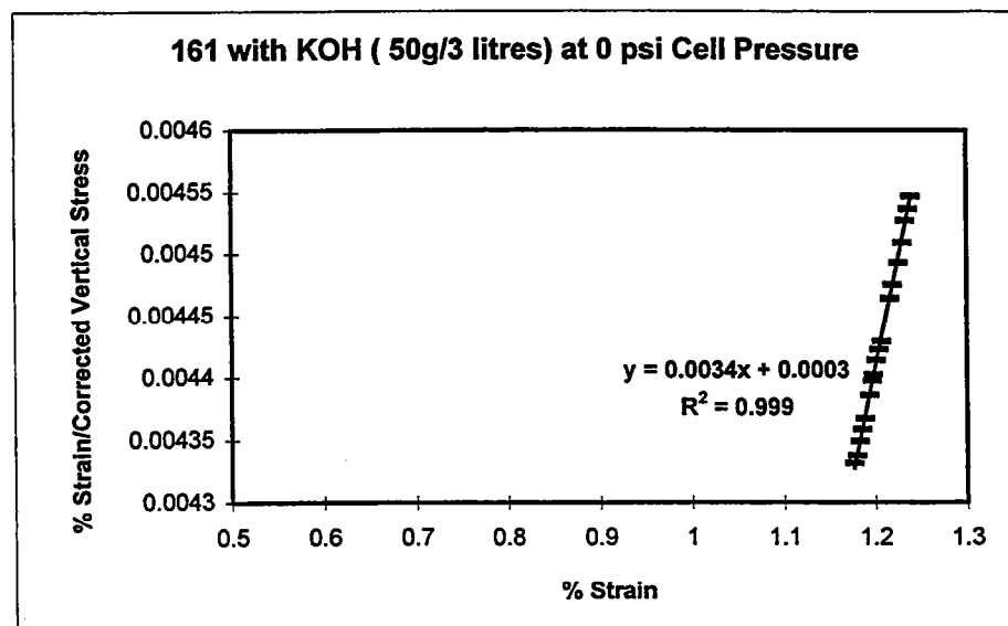
Figure 11. Modified Plot for KOH (50g/3ℓ) at 0 psi Cell Pressure (SH 161)
