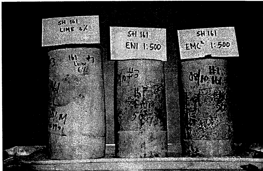
Figure 42. Photographs Showing Comparisons of Swell (Lime -6% Vs EN1-1:500, EMC 2 -1:500) - SH 161
