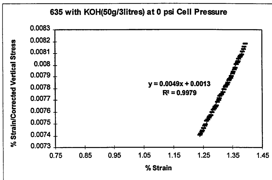
Figure 25. Modified Plot for KOH (50g/3ℓ) at 0 psi Cell Pressure (IH 635)
